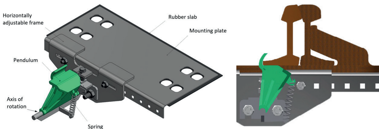
Bistable device. Cross section with switch rail in closed position (right picture).
