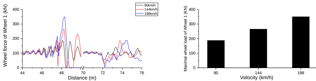
Figure 23. Wheel force of Wheel 1 in three cases: (a) Time history; (b) Maximum.
