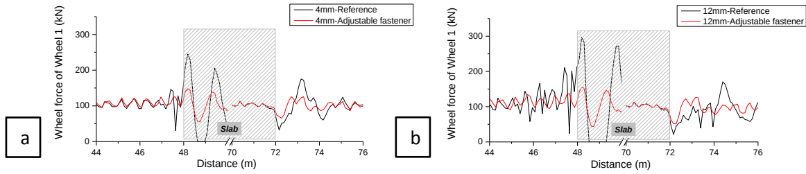
Figure 22. Wheel forces of the transition zones using adjustable fasteners: (a) 4mm differential settlement, (b) 12mm differential settlement.
