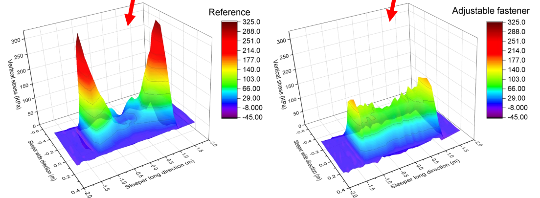
Ballast stress distribution under sleeper
