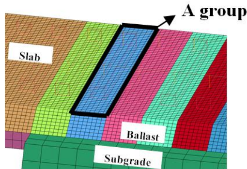
Figure 16. Collecting method for ballast stresses. Red lines are sleeper frames.
