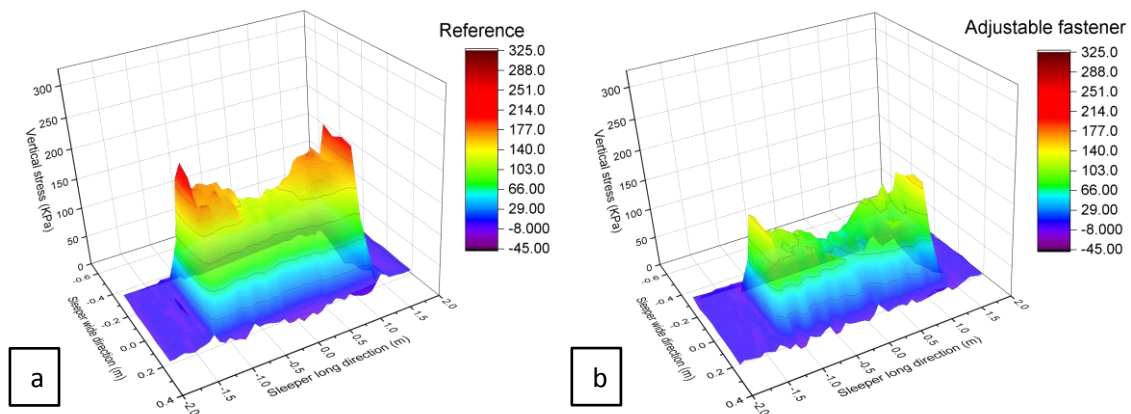
Figure 19. Stress distribution in ballast under Sleeper+3: (a) Reference case, (b) Using adjustable fasteners.
