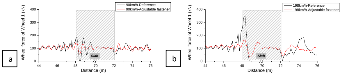
Figure 24. Wheel forces of the transition zones using adjustable fasteners: (a) 90km/h, (b) 198km/h.
