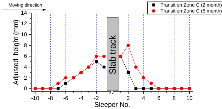
Figure 11. Adjusted heights of the fasteners in Transition Zone C.
