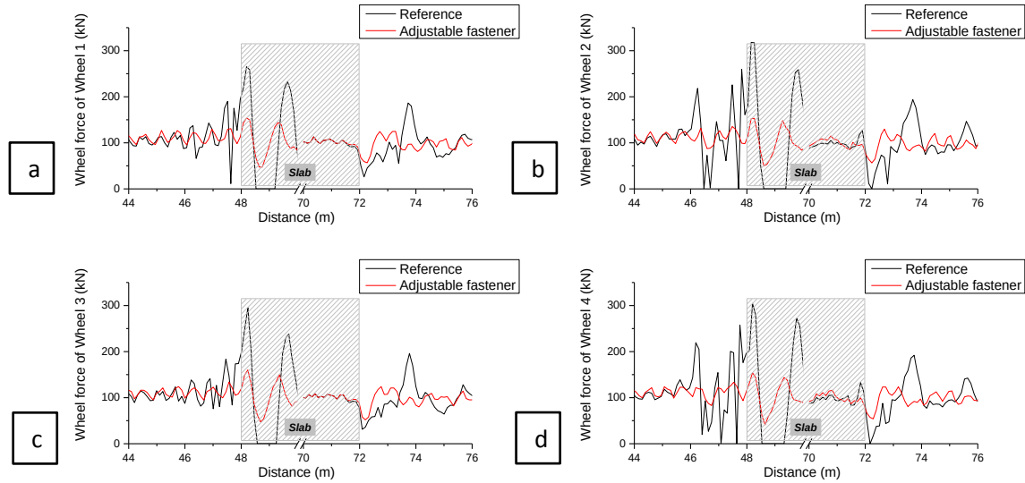
Figure 15. Wheel-rail interaction force of four wheelsets: (a) Wheel 1, (b) Wheel 2, (c) Wheel 3, (d) Wheel 4. The wheel loads on the slab track are covered by the shaded area.
