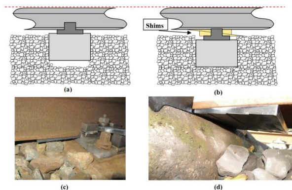
Figure 5. Schematic diagram of Adjustable fastener: (a)-(b) Working principle, (c)-(d) Examples of the adjustable fastener used in the track
