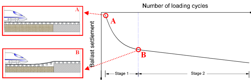
Figure 2. Schematic permanent settlement curve of ballast as a function of loading cycles (only for free ballast tracks).
