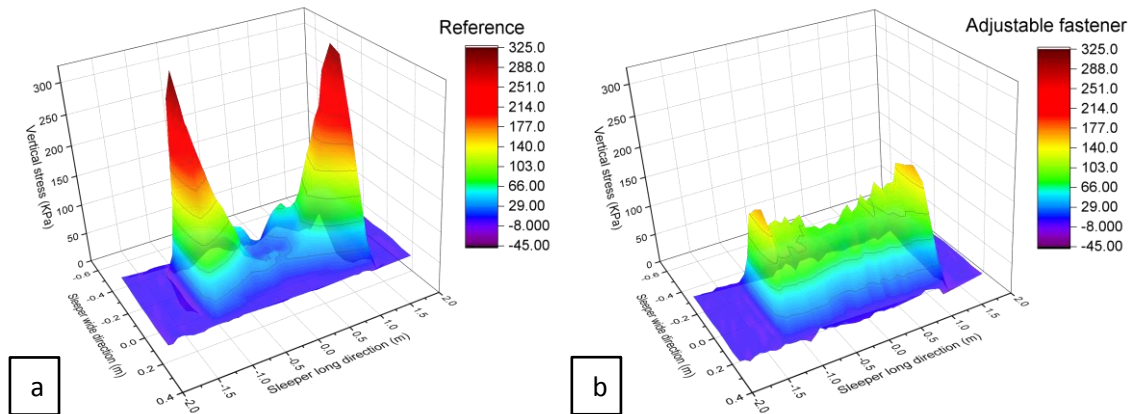
Figure 18. Stress distribution in ballast under Sleeper-2: (a) Reference case, (b) Using adjustable fasteners.
