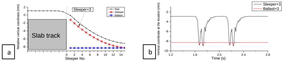
Figure 13: (a) Vertical coordinates of rail, sleepers and ballast due to 8 mm differential settlement; (b) Time history of vertical coordinate due to the passing vehicle at Sleeper+3.
