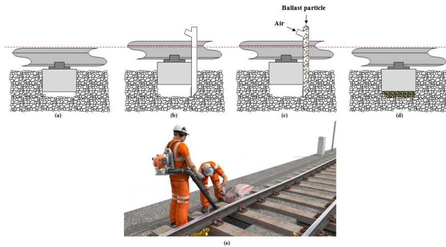
Figure 4. Schematic diagram of stone blowing: (a)-(d) Working principle, (e) is from Network Rail with permissions [45].
