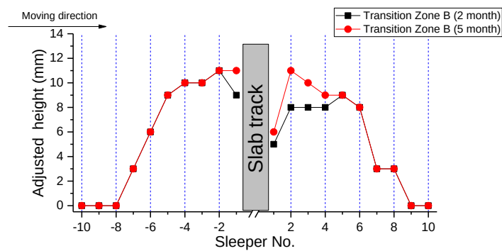
Figure 10. Adjusted heights of the fasteners in Transition Zone B.
