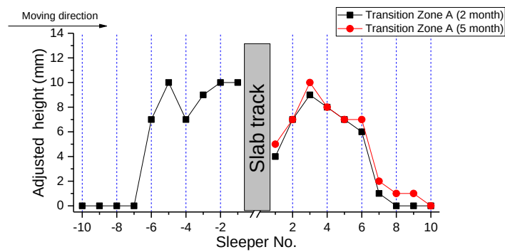
Figure 9. Adjusted heights of the fasteners in Transition Zone A.
