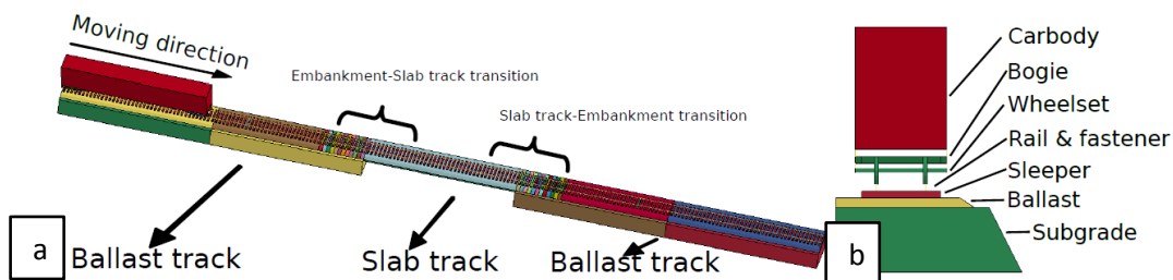
Figure 12. FE model of track transition zones: (a) Overview, (b) Side view.
