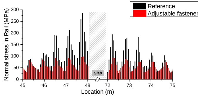
Figure 20. Normal stresses in rails in the reference case and the adjustable fastener case.
