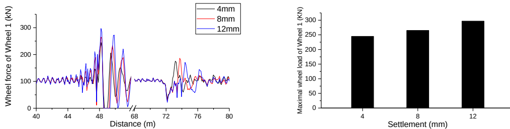
Figure 21. Wheel force of Wheel 1 in three cases: (a) Time history; (b) Maximum.
