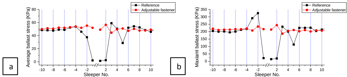
Figure 17. Ballast stresses along the track: (a) Average; (b) Maximal
