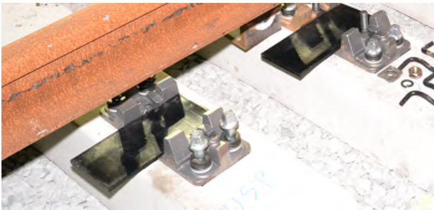
Figure 8 Fixing the ShimLift using existing bolts
